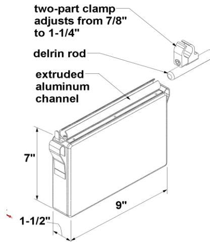
overall dimensions
